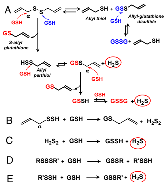
Fig. 5. H 2 S production from organic polysulfides by thiol reactions. (A) Proposed mechanism of H 2 S production by reaction of DADS and GSH via \alpha carbon nucleophilic attack (red); H 2 S is not produced by thiol/disulfide exchange (blue). (B) Nucleophilic substitution of allyl perthiol at the \alpha carbon followed by (C) thiol/disulfide exchange. (D and E) Thiol/disulfide exchange of organic trisulfides and higher polysulfides. See text below for description.
